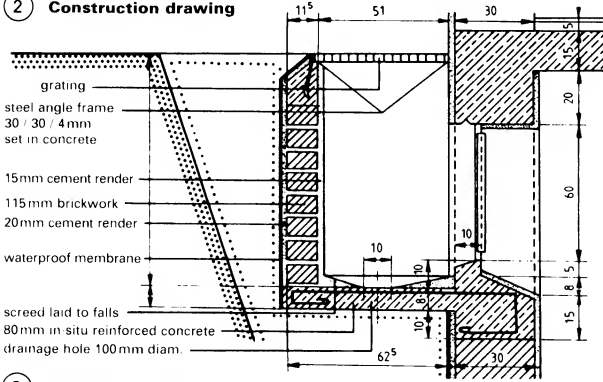
3 Detailed drawing
